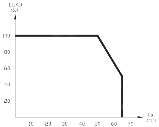
Derating curve
