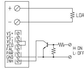
ON/OFF CONTROL BY TRANSISTOR
