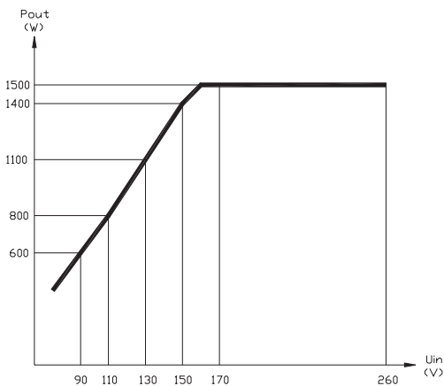
Output power vs Input voltage derating curve
